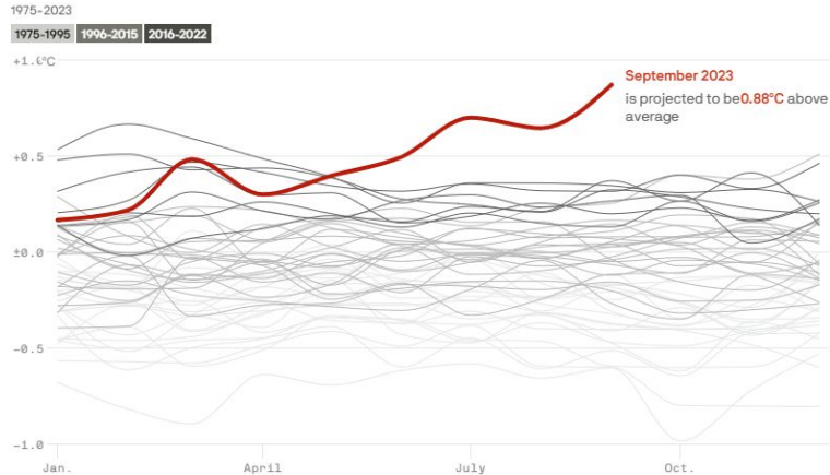
Monthly global temperature anomalies
